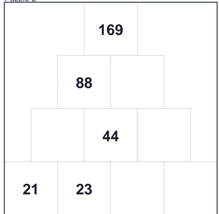
Puzzle 2
