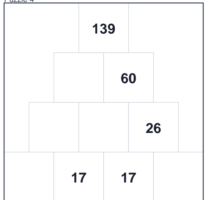
Puzzle 4
